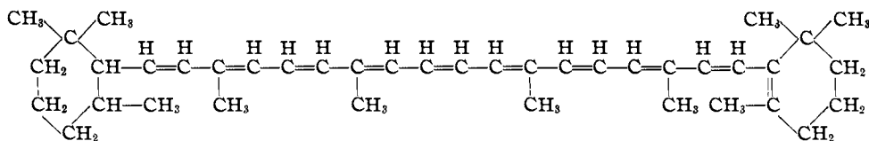
5,6-Dihydro- \beta -carotene
