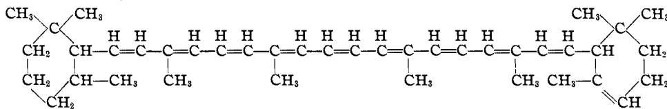
5,6-Dihydro- \alpha -carotene
